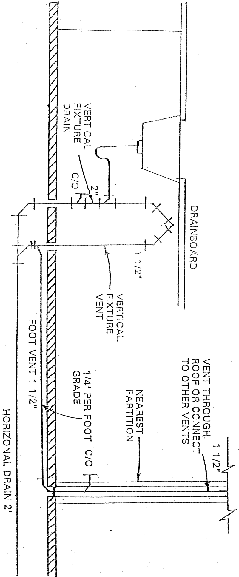
ACCEPTABLE ISLAND SINK INSTALLATION
